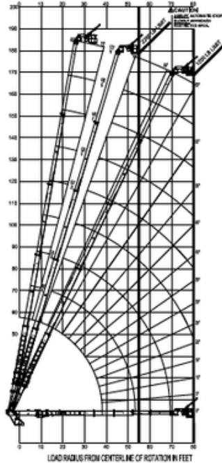
BOOM RANGE DIAGRAM WITH PLATFORM ATTACHED TO MAIN BOOM
